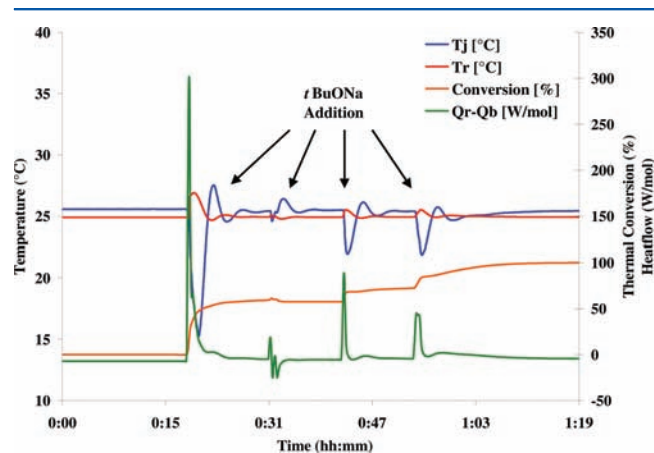
Figure 3. RC1 calorimetry of \alpha -arylation of 10: NaOt-Bu addition.
